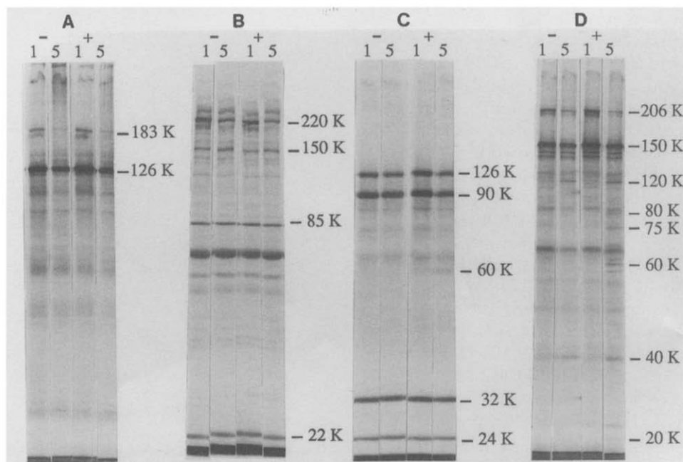
Fig. 3. Comparison of translation products of TMV (A), BNYVV (B), AIMV (C) and TYMV (D) RNAs in an untreated reticulocyte lysate (-) or supplemented with S micrococcal nuclease ( 5 \mu\text{g/ml} ) and unlabelled methionine ( 3 \text{ mM} ) after 45 min of incubation (+).
